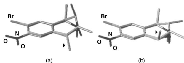
Figure 5. (a) Molecular modeling overlay of 16 , the most potent trans -7-nitro-THIQ, and 20 . The arrow indicates the 1-methyl moiety of 16 which shows the methyl group pointing below the plane of the THIQ nucleus. (b) Overlay of 17 , the least potent trans -7-nitro-THIQ, and 20 . The arrow indicates the 1-methyl moiety of 17 which shows the methyl group pointing out of the plane of the THIQ nucleus.
