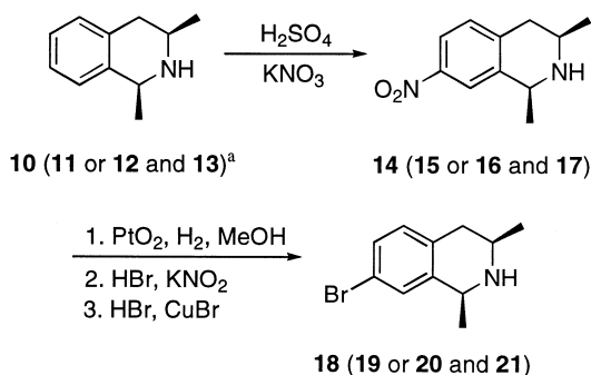
Scheme 2. a This synthesis scheme was repeated for compounds 11 and the racemic mixture of 12 and 13 .
