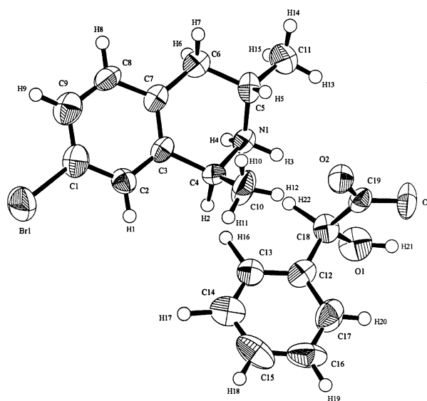
Figure 3. ORTEP diagram of the ( S )-(+)-mandelate salt of trans -(1 S ,3 S )- 21 . The atom numbering scheme agrees with the tables supplied in the supplemental material and thermal motion ellipsoids are shown at the 50% level.
