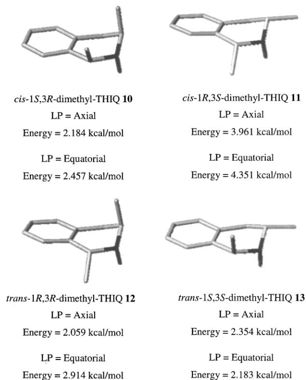
Figure 4. SYBYL-generated conformations and minimized energies for both cis - ( 10 and 11 ) and trans -1,3-dimethyl-1,2,3,4-tetrahydroisoquinolines ( 12 and 13 ). The starting coordinates for trans -1,3-dimethyl-THIQ 13 were taken from the X-ray crystal structure of 21 (Fig. 3) and the geometry optimized using the Tripos force field.
