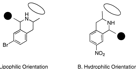
Figure 2. 1,3-Dimethyl-7-substituted-THIQs shown in the proposed lipophilic and hydrophilic binding orientation. According to this hypothesis the 1-methyl moiety will occupy different regions in space (depicted by the black circles), which have not been previously examined, depending upon the orientation of the molecule. The white ellipse shows the similar region of space occupied by the 3-methyl moiety in both orientations.
