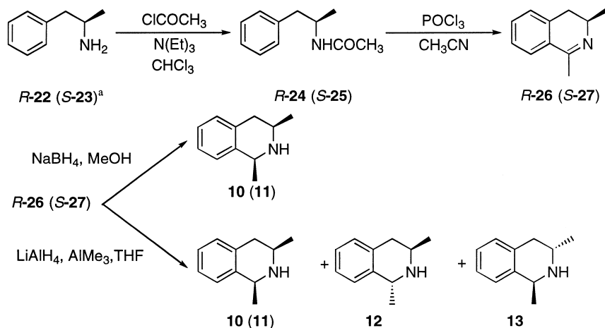
Scheme 1. a This reaction scheme was repeated for phenylpropylamine ( S -23) and the products of this synthesis are shown in parentheses.
